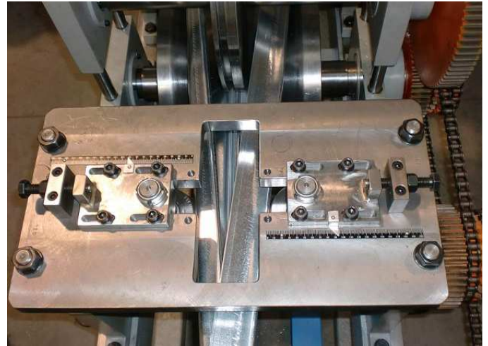
Roll-forming unity
