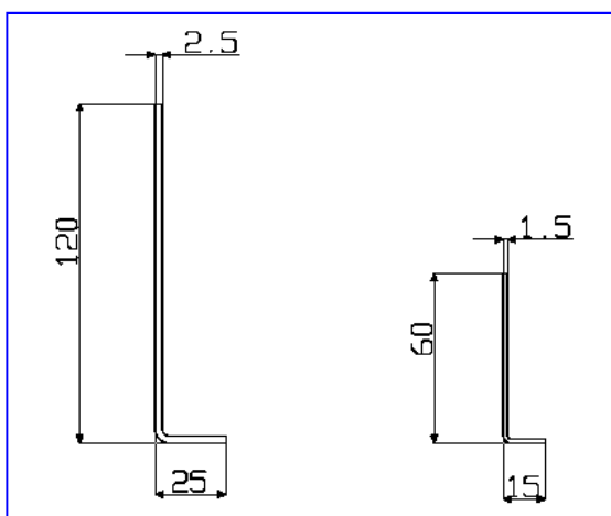
Max / min section of profile
