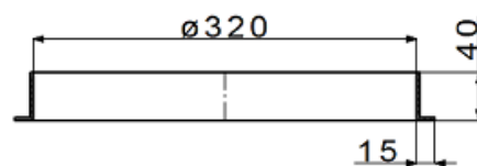
MIN RING
